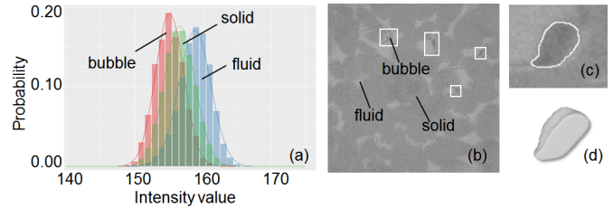
Fig. 3: Bubble detection and porous surface extraction. (a) Histogram of three phases in one bubble region of the XCT image. (b) Bubble detection (white rectangle) (Sect. 3(1)) and (c) precise segmentation (Fig. 3(2)). (d) Rendering of a 3D reconstruction.
